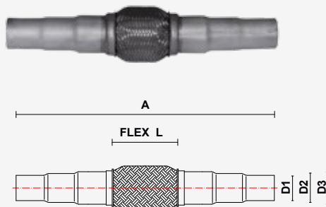
IMG 2 - Tubo flexible malla interior ajustable
